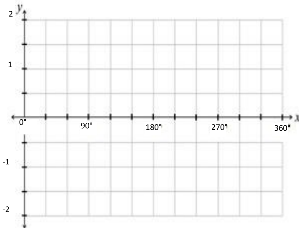
Sine and Cosecant
